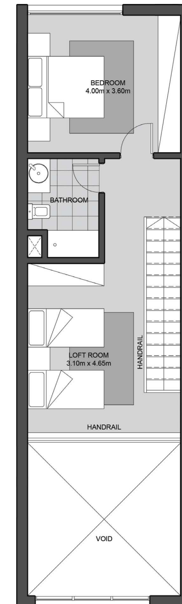
First Floor
